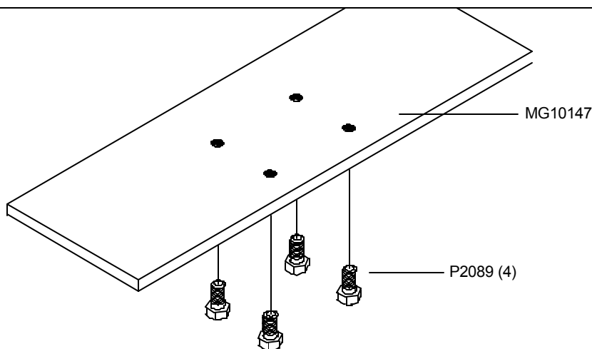
Figure 24 - SMK4 Dual-Head Mounting Plate Assembly
